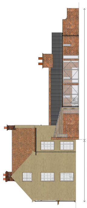
Elevation CC 1:100@A1
